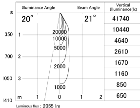
■ Direct Horizontal Illuminance DD140-2020MW9035D
