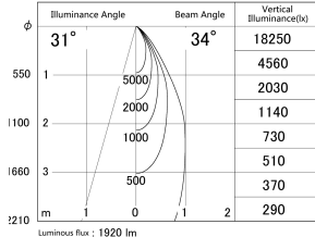
■ Direct Horizontal Illuminance DD140-2030MW9035D
