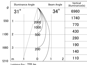
■ Direct Horizontal Illuminance DD140-0830MW9040D
