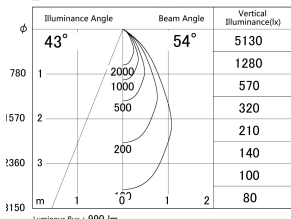
■ Direct Horizontal Illuminance DD140-1050MW9040D
