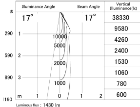
■ Direct Horizontal Illuminance DD140-1515MW9040D
