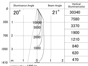
■ Direct Horizontal Illuminance DD140-1520MW9040D
