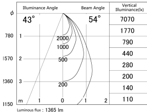
■ Direct Horizontal Illuminance DD140-1550MW9040D
