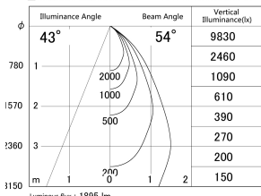
■ Direct Horizontal Illuminance DD140-2050MB9030D
