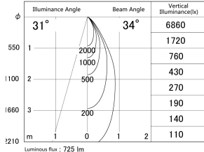
■ Direct Horizontal Illuminance DD140-0830MB9035D
