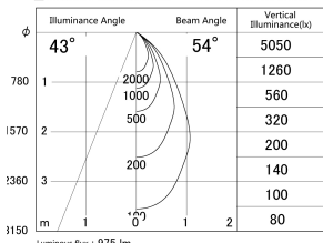
■ Direct Horizontal Illuminance DD140-1050MB9035D
