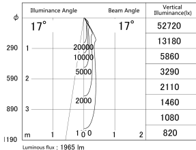
■ Direct Horizontal Illuminance DD140-2015MB9035D
