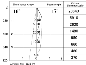
■ Direct Horizontal Illuminance DD140-1015DW9027D
