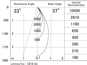
■ Direct Horizontal Illuminance DD140-1530DW9027D
