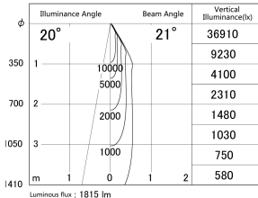
■ Direct Horizontal Illuminance DD140-2020DW9027D
