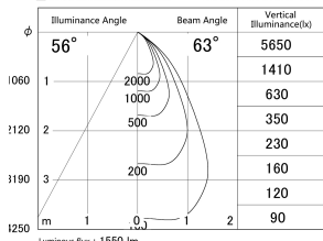
■ Direct Horizontal Illuminance DD140-2050DW9027D
