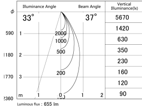
■ Direct Horizontal Illuminance DD140-0830DW9030D
