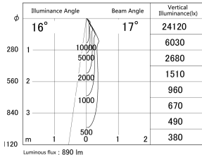
■ Direct Horizontal Illuminance DD140-1015DW9030D
