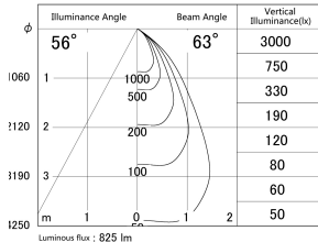
■ Direct Horizontal Illuminance DD140-1050DW9030D
