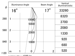
■ Direct Horizontal Illuminance DD140-1515DW9030D
