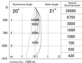
■ Direct Horizontal Illuminance DD140-1520DW9030D
