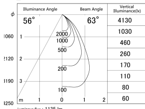
■ Direct Horizontal Illuminance DD140-1550DW9030D
