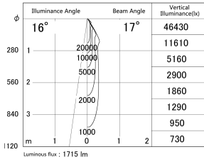
■ Direct Horizontal Illuminance DD140-2015DW9030D
