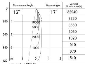
■ Direct Horizontal Illuminance DD140-1515DW9035D
