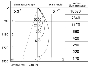
■ Direct Horizontal Illuminance DD140-1530DW9035D
