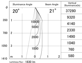
■ Direct Horizontal Illuminance DD140-2020DW9035D
