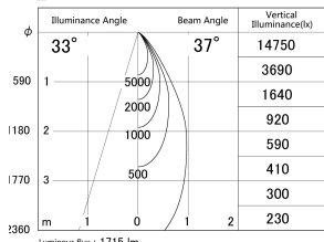
■ Direct Horizontal Illuminance DD140-2030DW9035D
