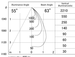
■ Direct Horizontal Illuminance DD140-0850DW9040D
