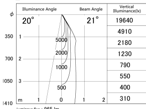
■ Direct Horizontal Illuminance DD140-1020DW9040D
