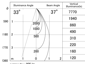
■ Direct Horizontal Illuminance DD140-1030DW9040D
