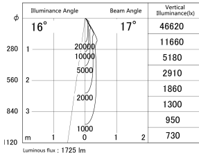
■ Direct Horizontal Illuminance DD140-2015DW9040D
