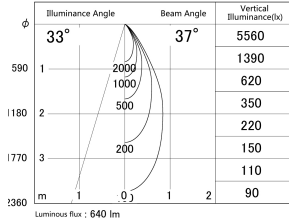
■ Direct Horizontal Illuminance DD140-0830DB9027D
