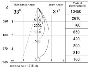
■ Direct Horizontal Illuminance DD140-1530DB9027D
