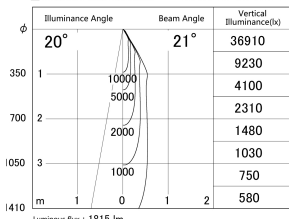
■ Direct Horizontal Illuminance DD140-2020DB9027D
