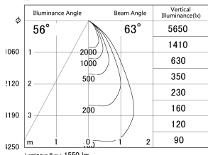
■ Direct Horizontal Illuminance DD140-2050DB9027D
