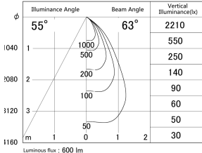
■ Direct Horizontal Illuminance DD140-0850DB9030D
