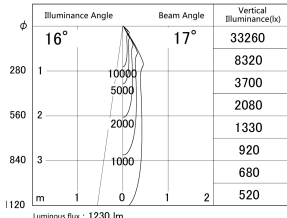
■ Direct Horizontal Illuminance DD140-1515DB9030D
