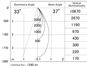
■ Direct Horizontal Illuminance DD140-1530DB9030D
