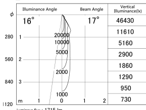
■ Direct Horizontal Illuminance DD140-2015DB9030D
