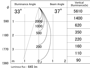
■ Direct Horizontal Illuminance DD140-0830DB9035D
