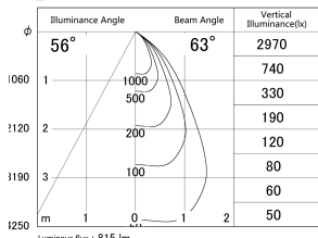
■ Direct Horizontal Illuminance DD140-1050DB9035D
