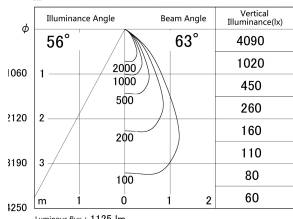
■ Direct Horizontal Illuminance DD140-1550DB9035D
