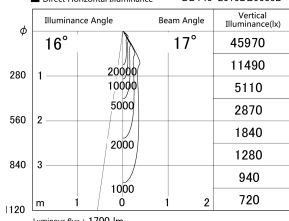
■ Direct Horizontal Illuminance DD140-2015DB9035D
