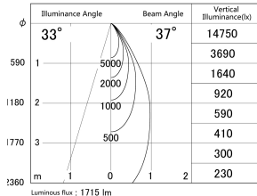
■ Direct Horizontal Illuminance DD140-2030DB9035D
