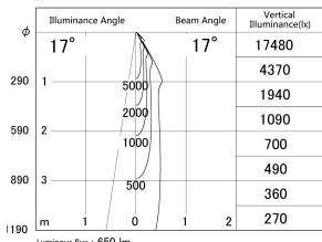
■ Direct Horizontal Illuminance DD140-0815DB9040D
