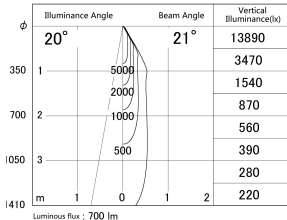
■ Direct Horizontal Illuminance DD140-0820DB9040D
