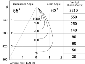
■ Direct Horizontal Illuminance DD140-0850DB9040D
