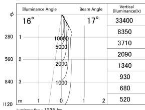
■ Direct Horizontal Illuminance DD140-1515DB9040D
