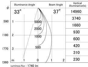
■ Direct Horizontal Illuminance DD140-2030DB9040D
