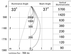
■ Direct Horizontal Illuminance DD140-0830WW9027D
