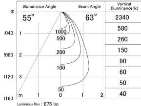
■ Direct Horizontal Illuminance DD140-0850WW9027D
